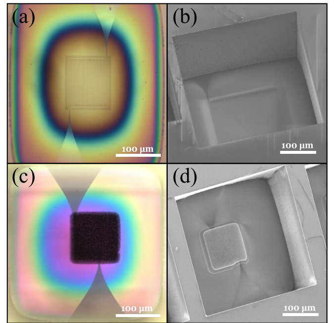
Figure 2. Optical and scanning-electron microscope (SEM) images of the membrane-style devices. (a) Optical image before VACNT growth, (b) SEM before VACNT growth, (c) optical image after VACNT growth and (d) SEM after VACNT growth.
