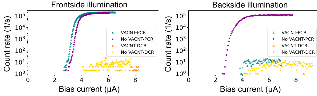
Figure 5. Photon count rates and dark count rates of membrane-style devices. PCR measurements taken using flood illumination at 980 nm. Measured same devices in two separate cooldowns. (left) frontside illumination and (right) backside illumination.
