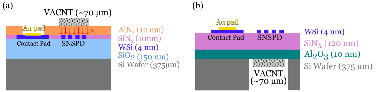
Figure 1. Cross-sectional view of the two fabrication processes for integrating VACNTs with SNSPDs. (a) Integrating VACNTs directly on the surface of the SNSPD, using a capping layer between them (b) Growing the VACNTs on the underside of a membrane-suspended SNSPD.
