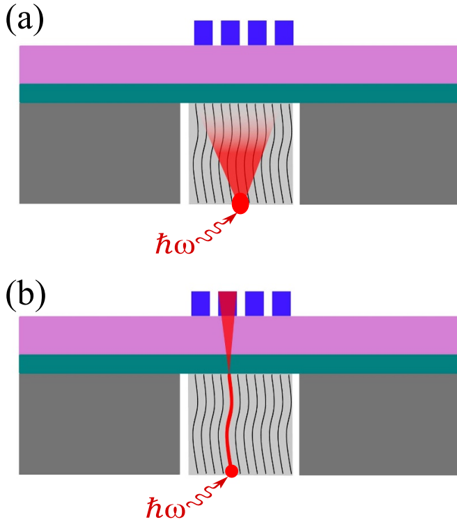
Figure 6. Potential heating dynamics in membrane style devices. (a) Phonons generated from photon absorption in a VACNT diffuse throughout VACNT forest volume. Once phonons reach the capping layer the energy is not localized enough to produce a hot-spot in the nanowire. (b) A single nanotube carries the deposited energy to the surface of the substrate. These phonons then travel through the capping layer to the nanowire in a localized fashion and induce a hot-spot in the nanowire. It must be noted that the thermal transport properties of carbon nanotubes will also depend on crystallinity, defects, temperature, density and temperature-dependent electron phonon mobility [24].
