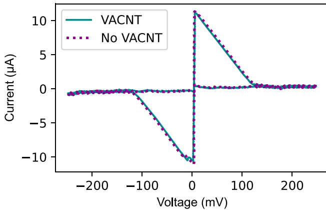
Figure 4. IV curves of membrane style SNSPDs with VACNTs (blue) and without (purple), showing that VACNTs could be integrated without reducing the current-carrying capacity of the SNSPD.
