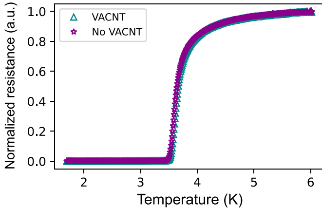
Figure 3. T_c measurement of a membrane-style device, showing that the VACNT growth process does not reduce the critical temperature of the SNSPD film. Plotting measured normalized resistance as a function of temperature before VACNT growth (purple) and after VACNT growth (blue).
